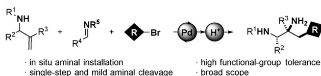
Scheme 1. Syntheses of diamines using a tether approach.
