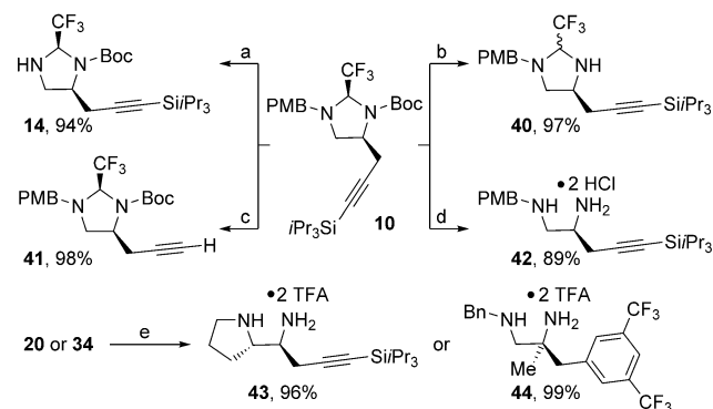
Scheme 3. Orthogonal deprotection. Reaction conditions: a) DDQ, MeCN, H_2O , RT; b) microwave irradiation (160°C), H_2O /Ethanol; c) TBAF, THF, 0°C to RT; d) HCl, MeOH, –40°C to RT; e) TFA, CH_2Cl_2 , then MeOH, 0°C to RT.
