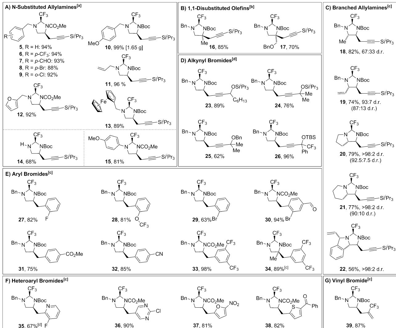
Scheme 2. Scope of the tandem amination-carboamination reaction. d.r. >20:1 unless otherwise noted; d.r. in parenthesis represents the diastereoisomeric ratio in the crude reaction mixture if different from the one of the isolated compound. [a] P(2-furyl) 3 (12 mol %) as ligand. [b] PhDavePhos (15–20 mol %) as ligand. [c] P(2-furyl) 3 (24 mol %) as ligand and cesium triflate as additive (1.2 equiv). [d] DPEPhos (12 mol %) as ligand.
